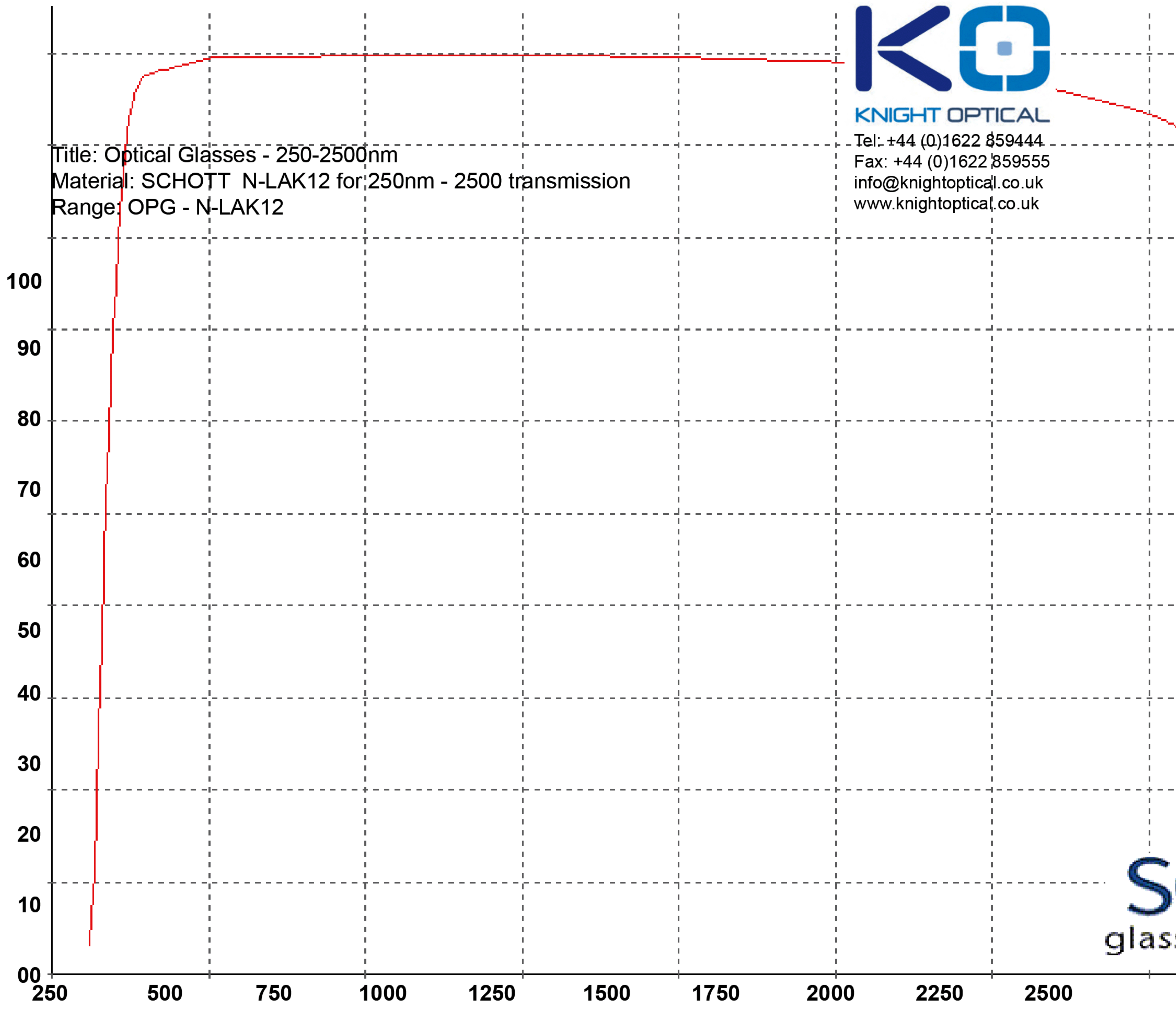
Wavelength in nm Internal transmittance for 10mm thickness
